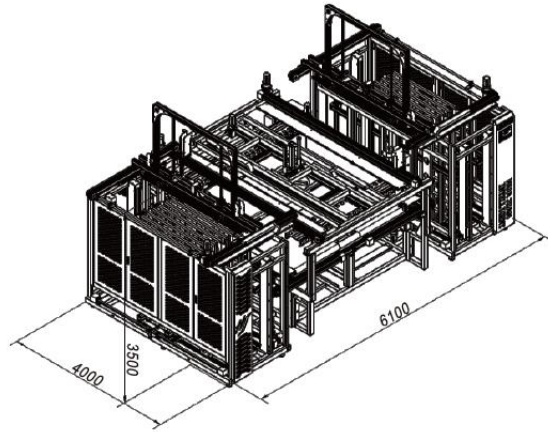
Foam Edge Gluing Machine FOAM TO FOAM
