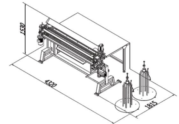
Bonnell Assembling Machine SX-200S
