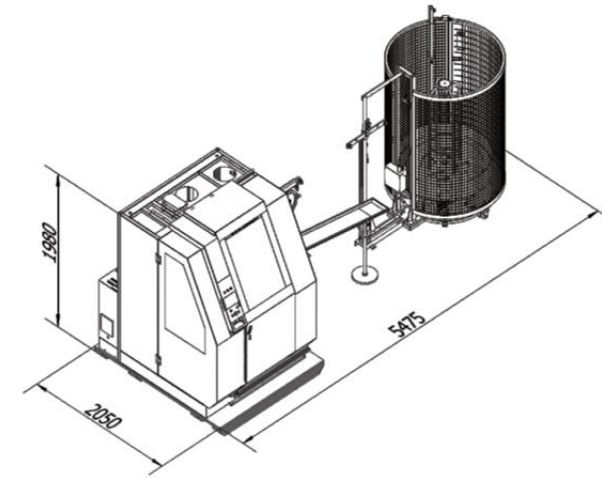
Bonnell Assembling Machine SX-200S
