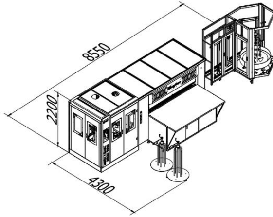
Bonnell Transfer Line STANDARD
