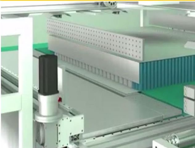
Foam Edge Gluing Machine 80–240 MM HEIGHT
