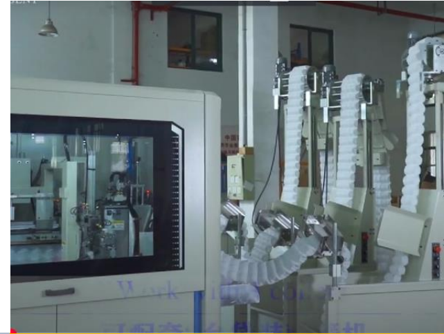
Pocket Spring Assembly Machine 6 COILERS
