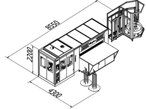
Bonnell Transfer Line OPEN COIL
