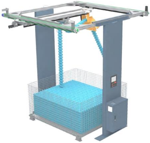
Auxiliary Equipment SX-1 BEFORE SX-300DL
